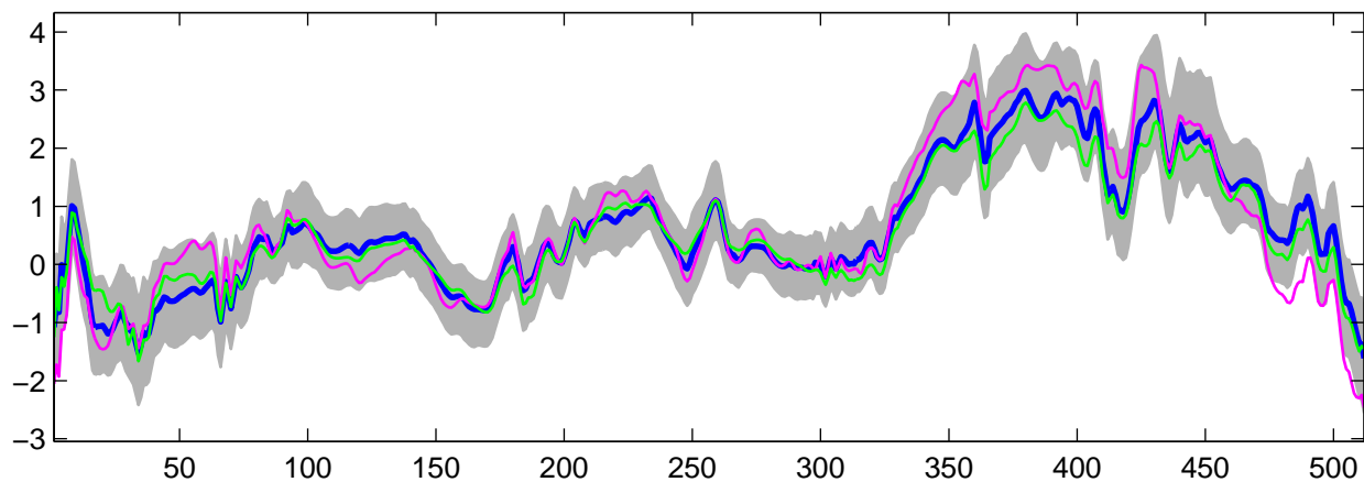
Estimated U_{17}(t) using R-WFMM: Normal data, run 2
