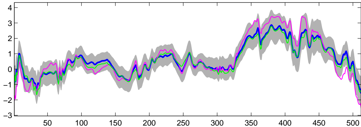
Estimated U_{17}(t) using G-WFMM: Normal data, run 2
