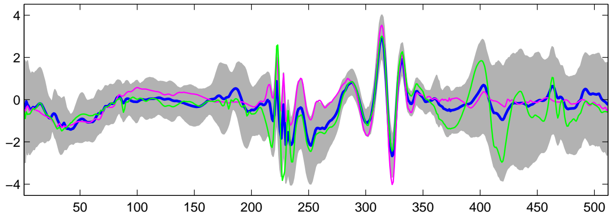
Estimated U_{17}(t) using G-WFMM: t_1 data, run 2
