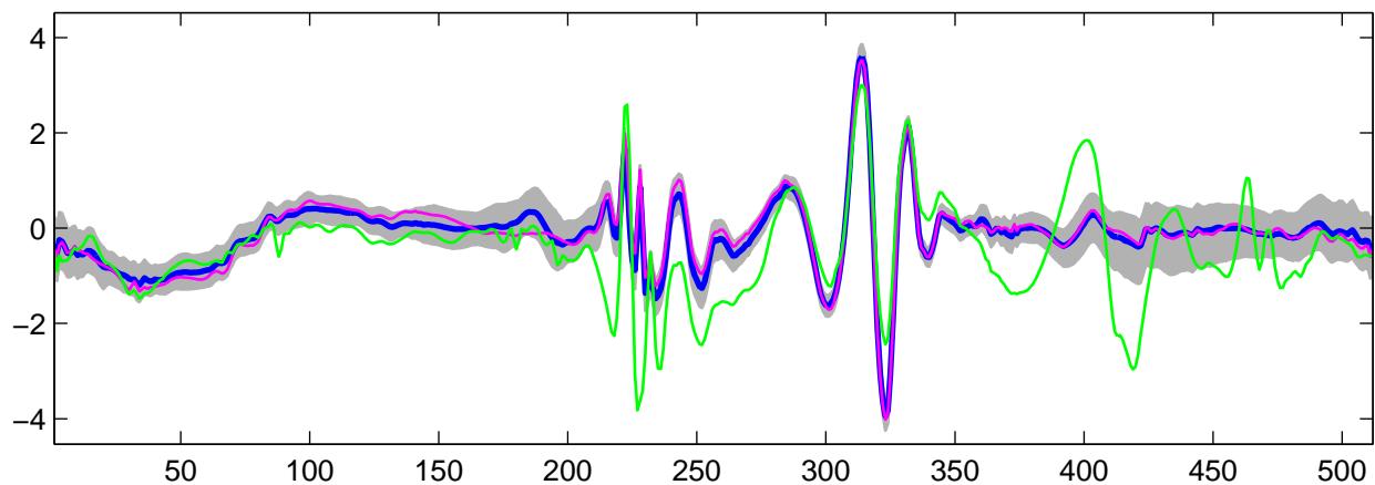
Estimated U_{17}(t) using R-WFMM: t_1 data, run 2
