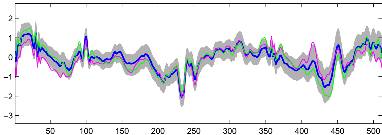
Estimated U_{17}(t) using R-WFMM: t_3 data, run 2
