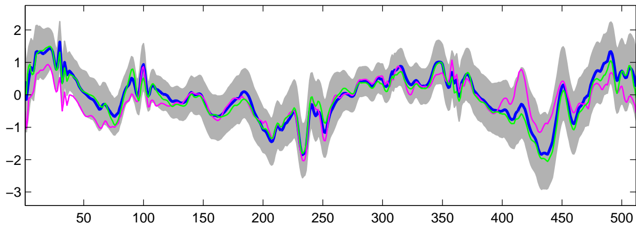
Estimated U_{17}(t) using G-WFMM: t_3 data, run 2
