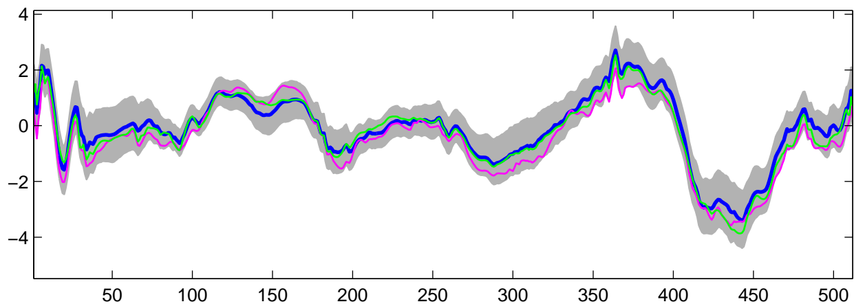
Estimated U_{18}(t) using R-WFMM: DE data, run 2
