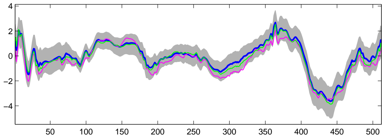
Estimated U_{18}(t) using G-WFMM: DE data, run 2
