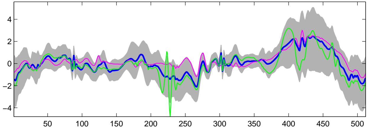
Estimated U_{18}(t) using G-WFMM: t_1 data, run 2
