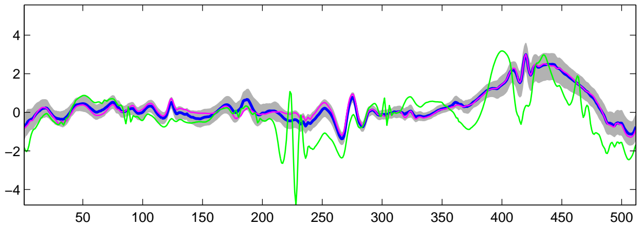
Estimated U_{18}(t) using R-WFMM: t_1 data, run 2
