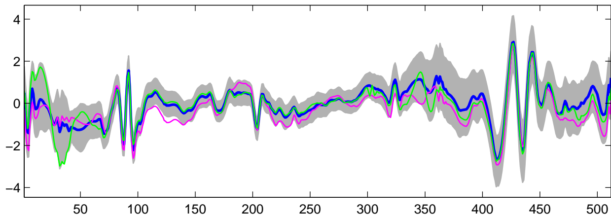
Estimated U_{18}(t) using G-WFMM: t_2 data, run 2
