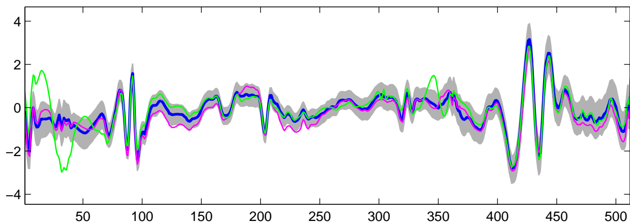
Estimated U_{18}(t) using R-WFMM: t_2 data, run 2
