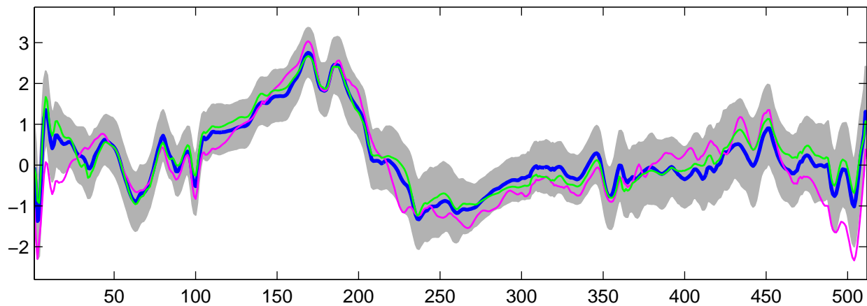
Estimated U_{19}(t) using G-WFMM: t_3 data, run 2
