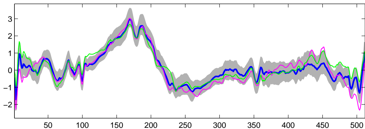
Estimated U_{19}(t) using R-WFMM: t_3 data, run 2
