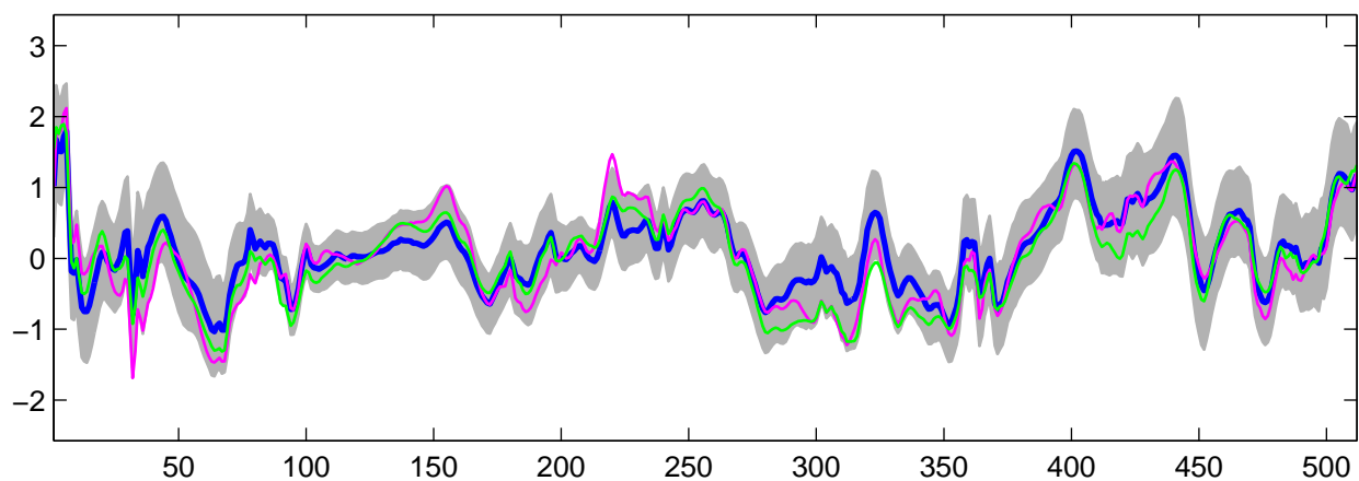
Estimated U_1(t) using R-WFMM: DE data, run 2
