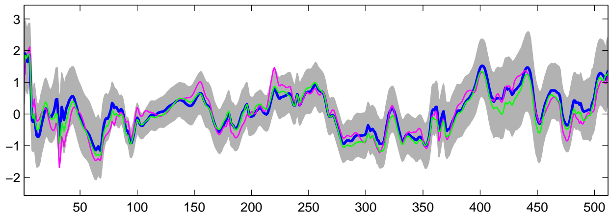
Estimated U_1(t) using G-WFMM: DE data, run 2
