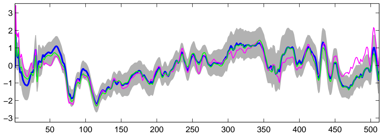
Estimated U_1(t) using R-WFMM: Normal data, run 2
