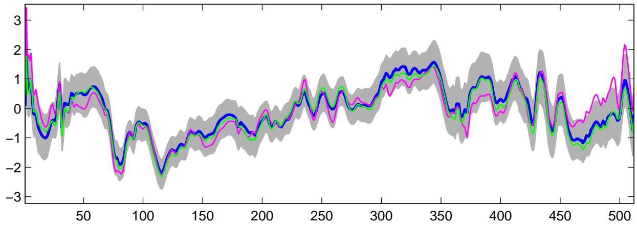
Estimated U_1(t) using G-WFMM: Normal data, run 2
