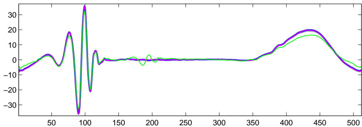
Estimated U_1(t) using R-WFMM: t_1 data, run 2
