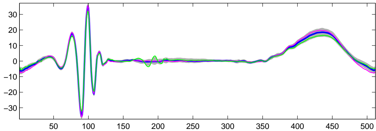
Estimated U_1(t) using G-WFMM: t_1 data, run 2
