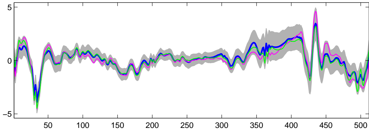
Estimated U_1(t) using G-WFMM: t_2 data, run 2
