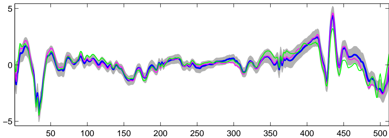
Estimated U_1(t) using R-WFMM: t_2 data, run 2
