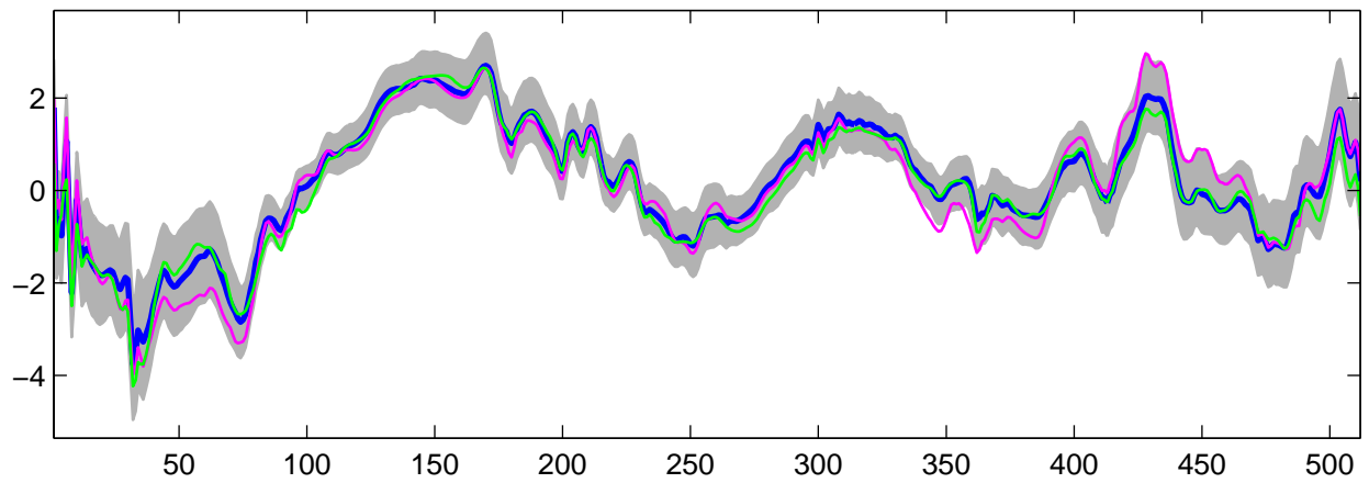
Estimated U_{20}(t) using R-WFMM: DE data, run 2
