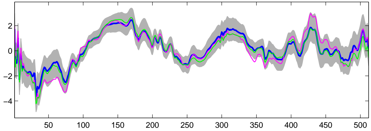
Estimated U_{20}(t) using G-WFMM: DE data, run 2
