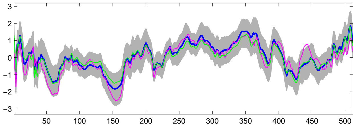
Estimated U_{20}(t) using G-WFMM: Normal data, run 2
