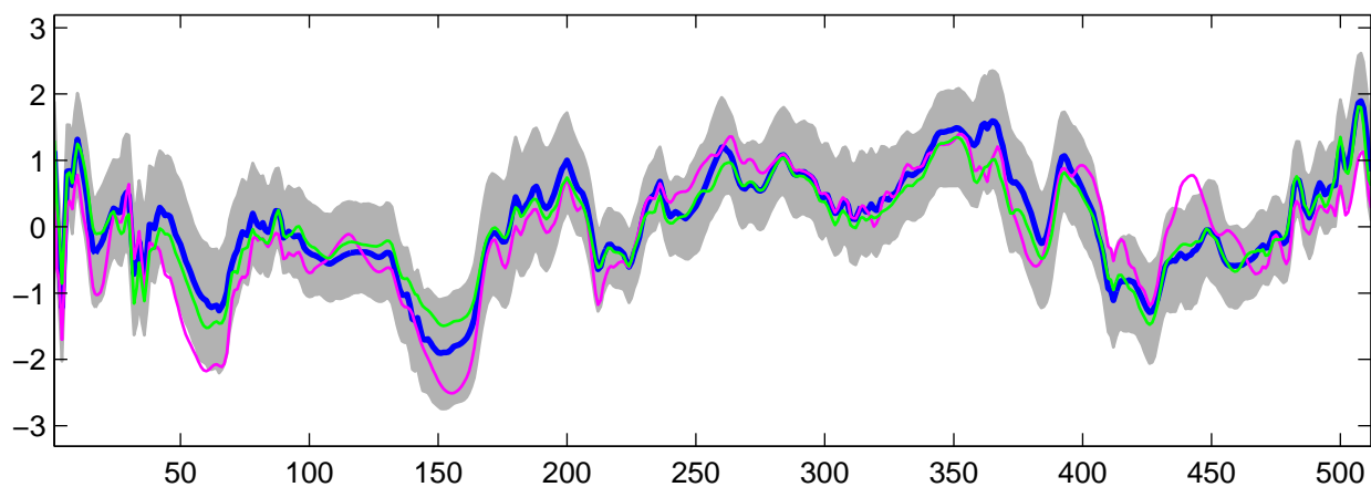
Estimated U_{20}(t) using R-WFMM: Normal data, run 2
