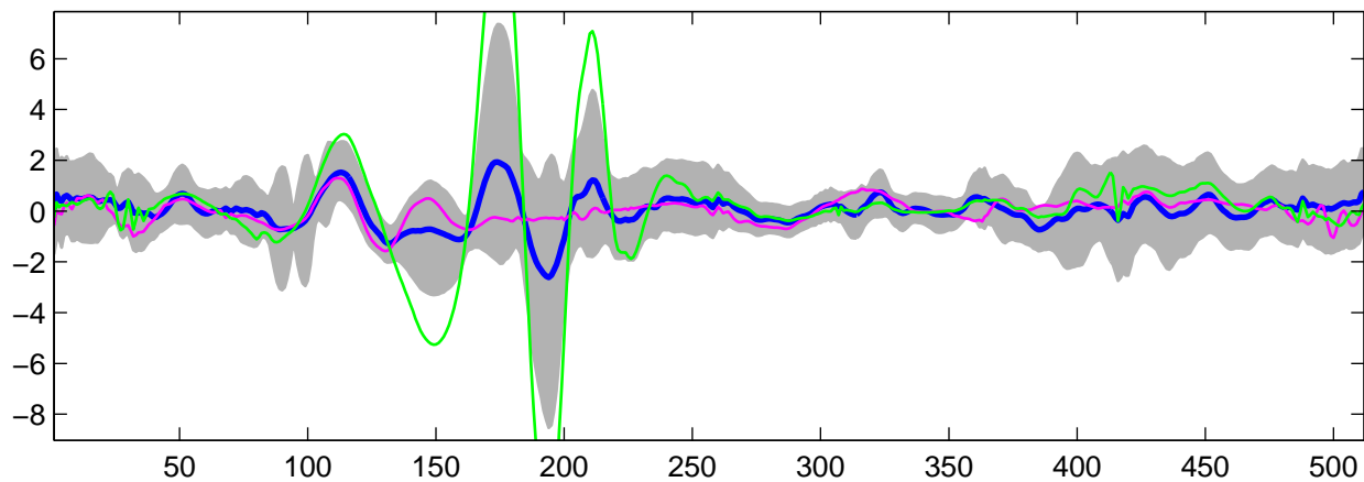
Estimated U_{20}(t) using G-WFMM: t_1 data, run 2
