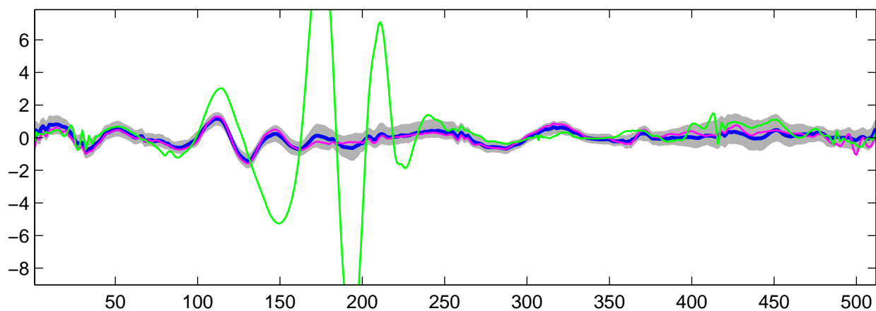
Estimated U_{20}(t) using R-WFMM: t_1 data, run 2
