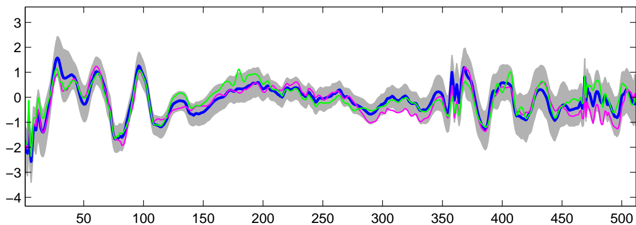
Estimated U_{20}(t) using R-WFMM: t_2 data, run 2
