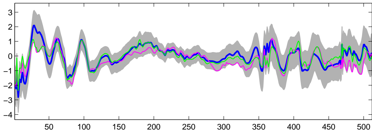
Estimated U_{20}(t) using G-WFMM: t_2 data, run 2
