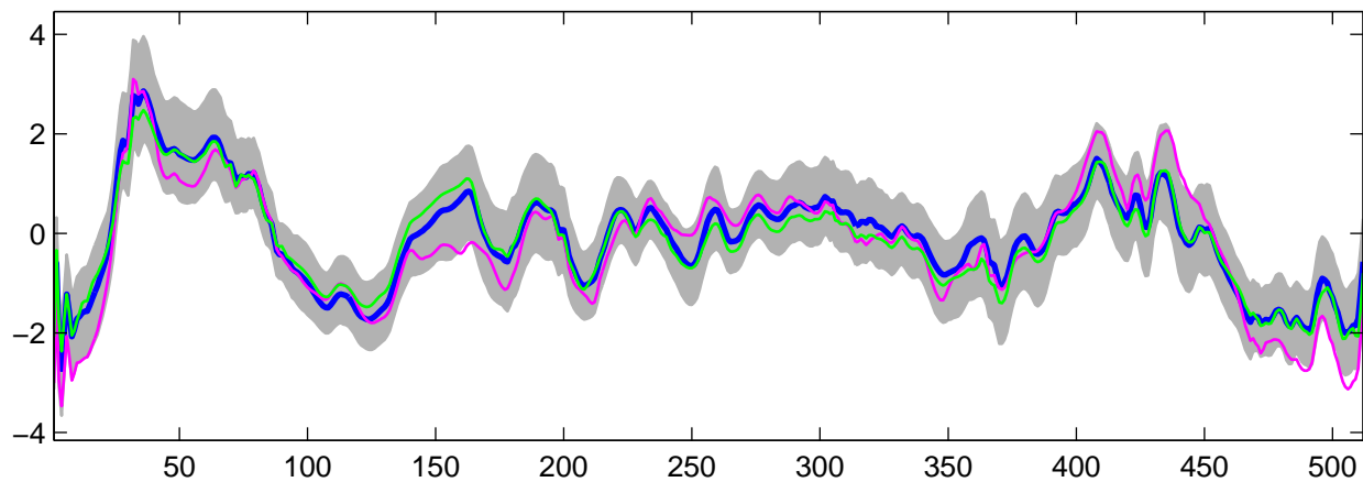
Estimated U_{21}(t) using G-WFMM: Normal data, run 2
