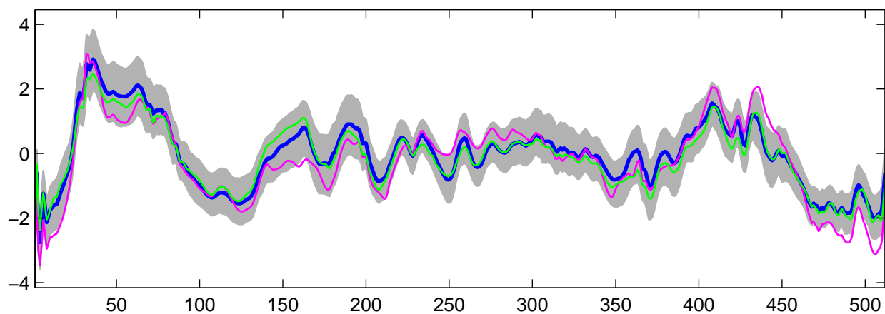
Estimated U_{21}(t) using R-WFMM: Normal data, run 2
