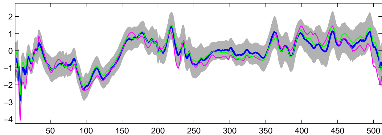
Estimated U_{21}(t) using G-WFMM: t_3 data, run 2
