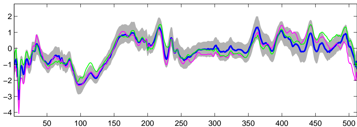
Estimated U_{21}(t) using R-WFMM: t_3 data, run 2
