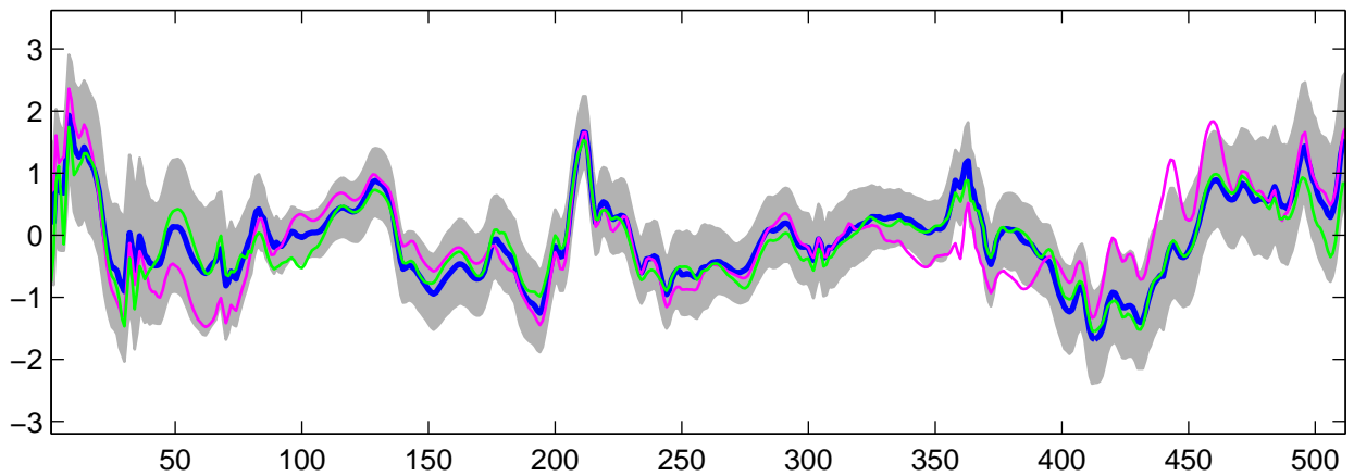
Estimated U_{22}(t) using R-WFMM: DE data, run 2
