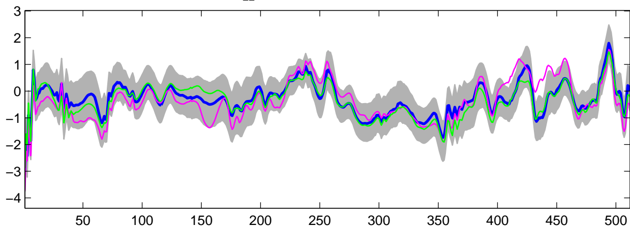
Estimated U_{22}(t) using R-WFMM: Normal data, run 2
