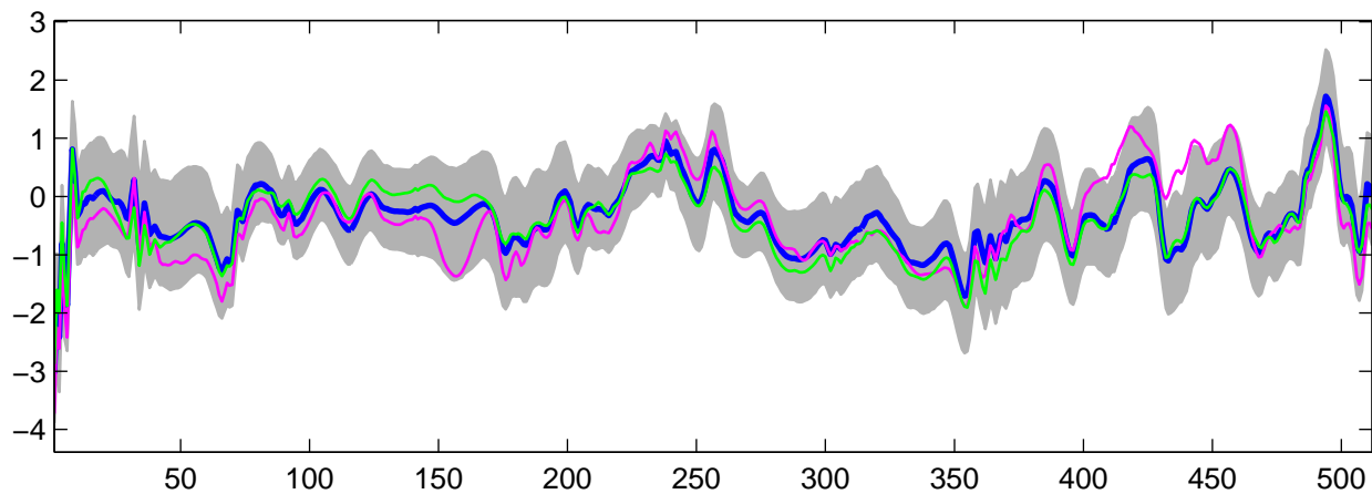
Estimated U_{22}(t) using G-WFMM: Normal data, run 2
