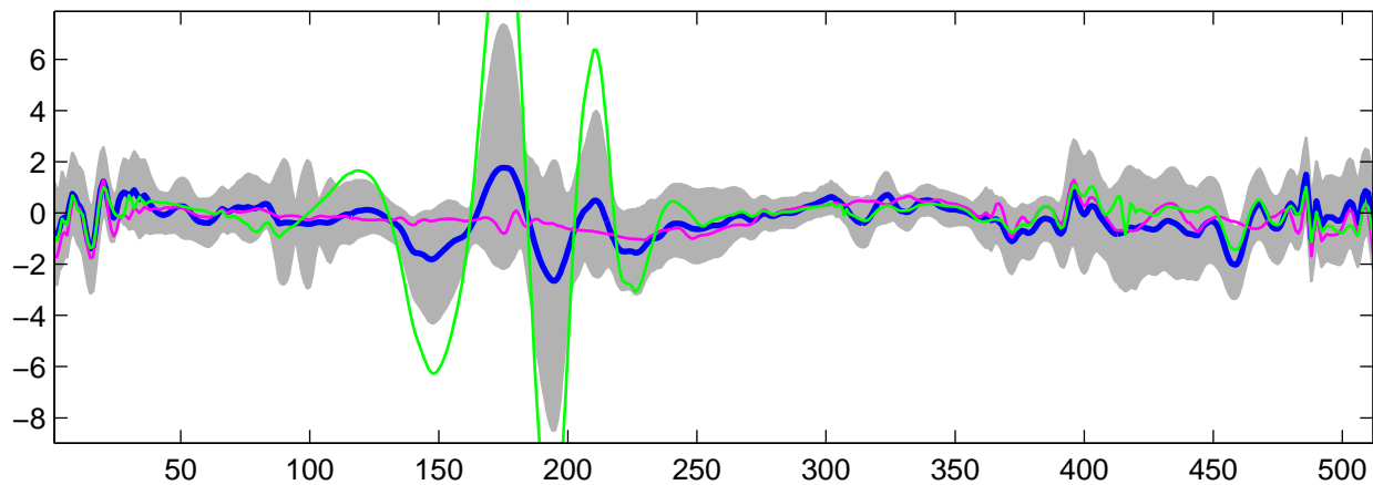
Estimated U_{22}(t) using G-WFMM: t_1 data, run 2
