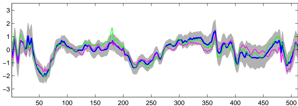
Estimated U_{22}(t) using R-WFMM: t_2 data, run 2
