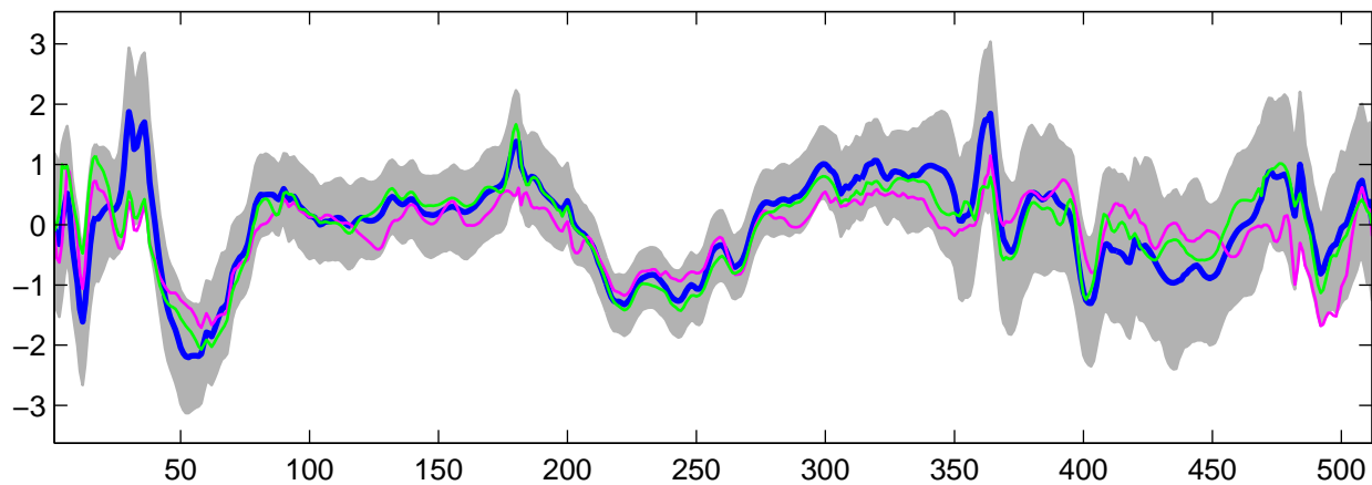
Estimated U_{22}(t) using G-WFMM: t_2 data, run 2
