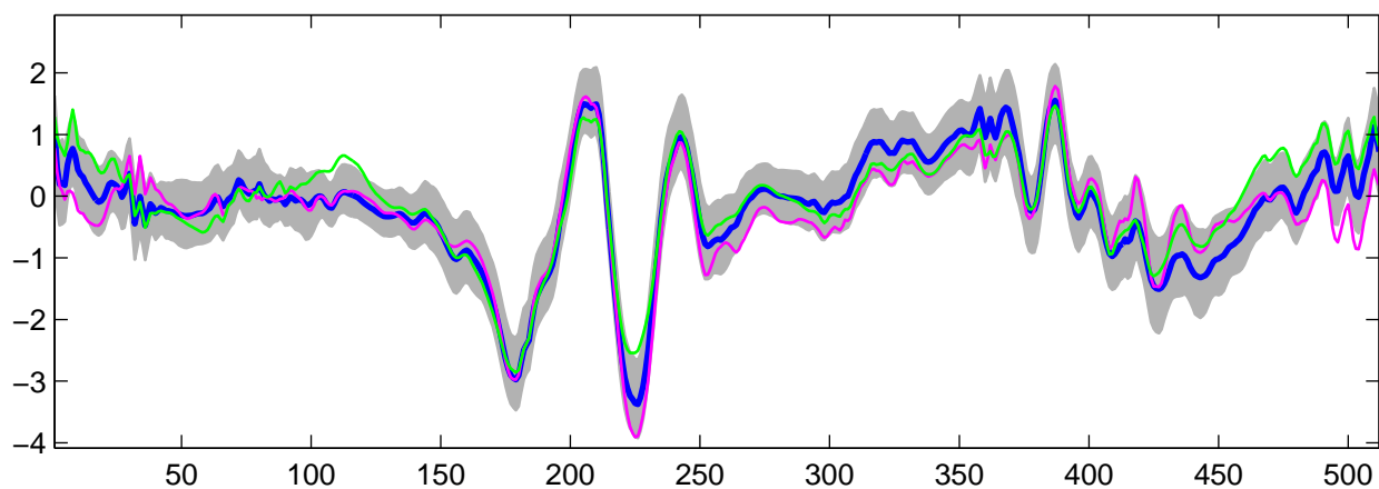
Estimated U_{22}(t) using R-WFMM: t_3 data, run 2
