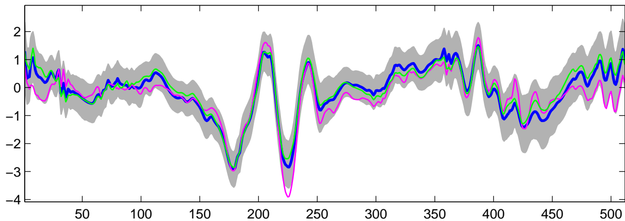
Estimated U_{22}(t) using G-WFMM: t_3 data, run 2
