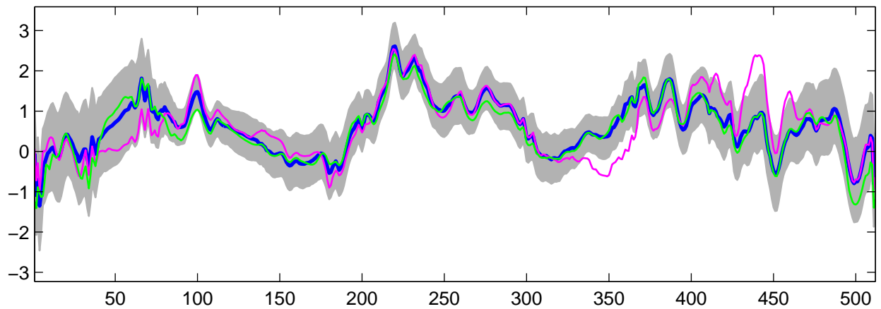
Estimated U_{23}(t) using R-WFMM: DE data, run 2
