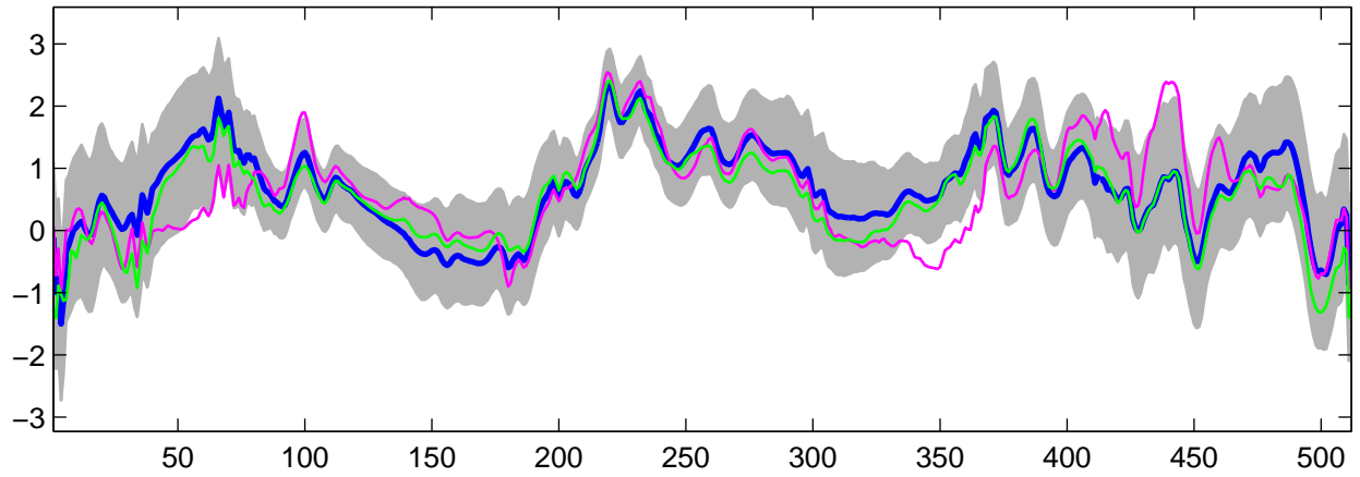
Estimated U_{23}(t) using G-WFMM: DE data, run 2
