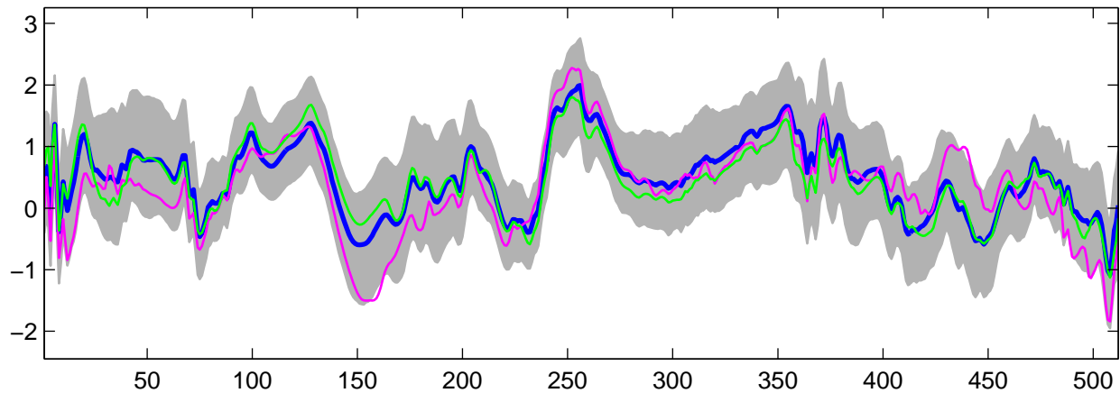
Estimated U_{23}(t) using G-WFMM: Normal data, run 2
