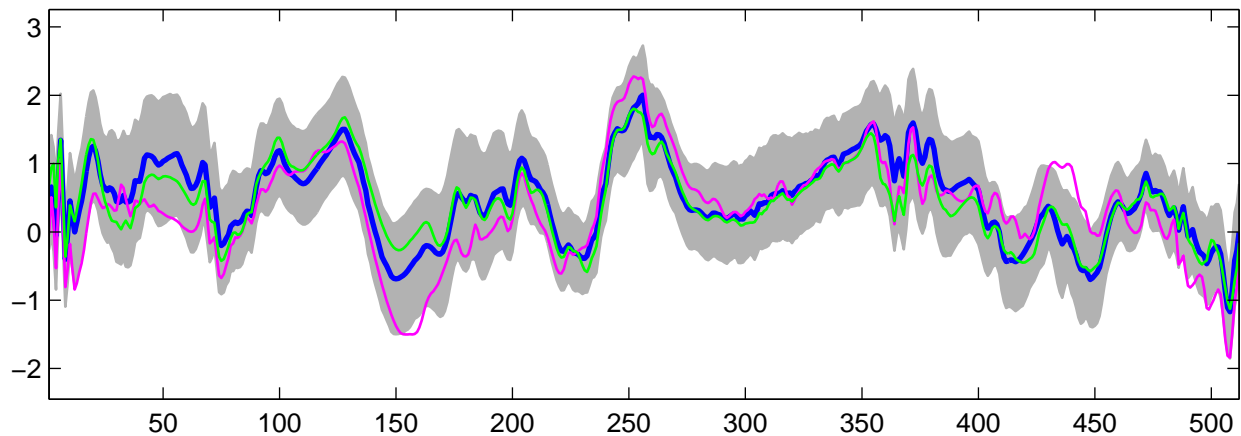
Estimated U_{23}(t) using R-WFMM: Normal data, run 2
