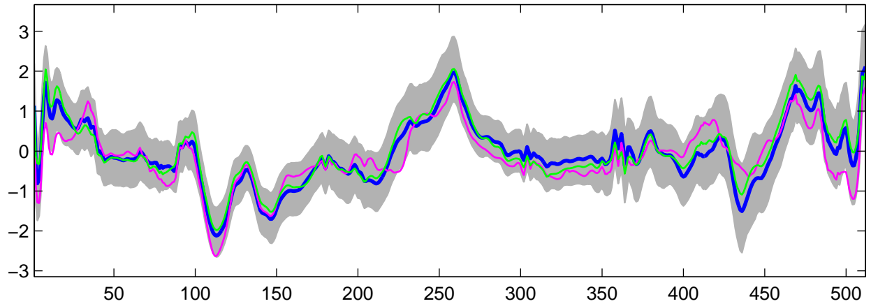
Estimated U_{23}(t) using G-WFMM: t_3 data, run 2
