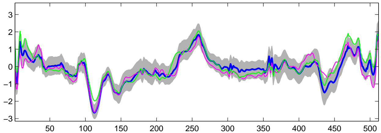
Estimated U_{23}(t) using R-WFMM: t_3 data, run 2
