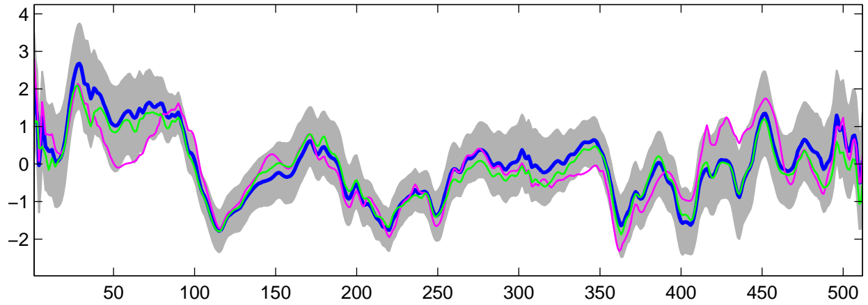
Estimated U_{24}(t) using G-WFMM: DE data, run 2
