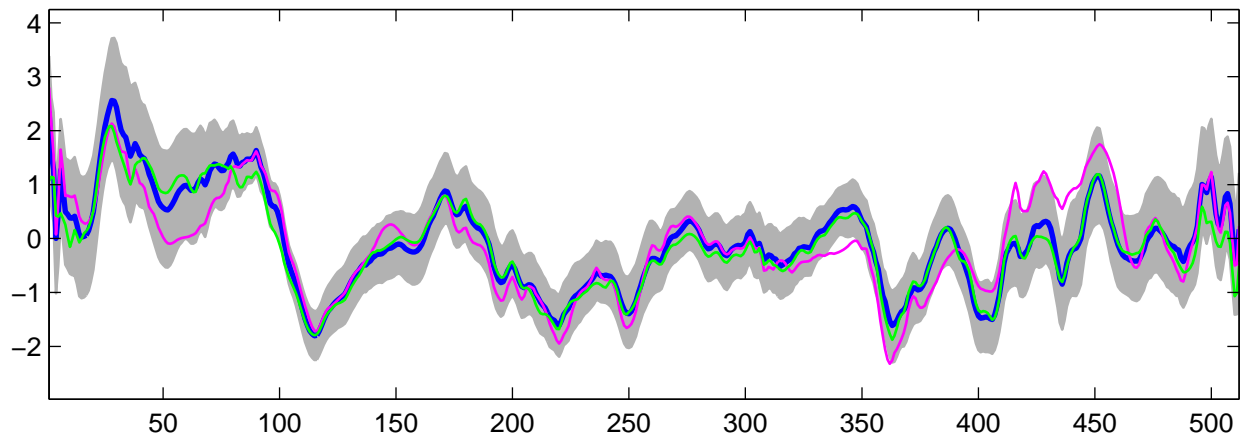
Estimated U_{24}(t) using R-WFMM: DE data, run 2
