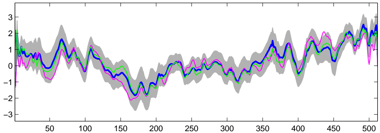
Estimated U_{24}(t) using R-WFMM: Normal data, run 2
