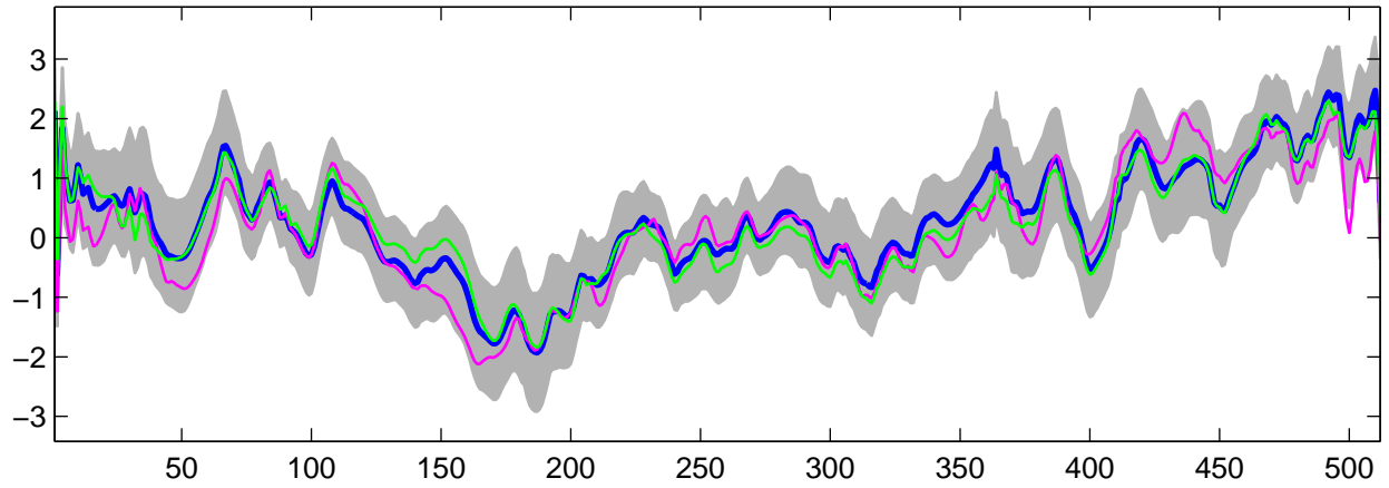
Estimated U_{24}(t) using G-WFMM: Normal data, run 2
