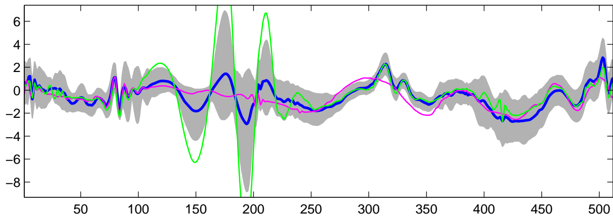
Estimated U_{24}(t) using G-WFMM: t_1 data, run 2
