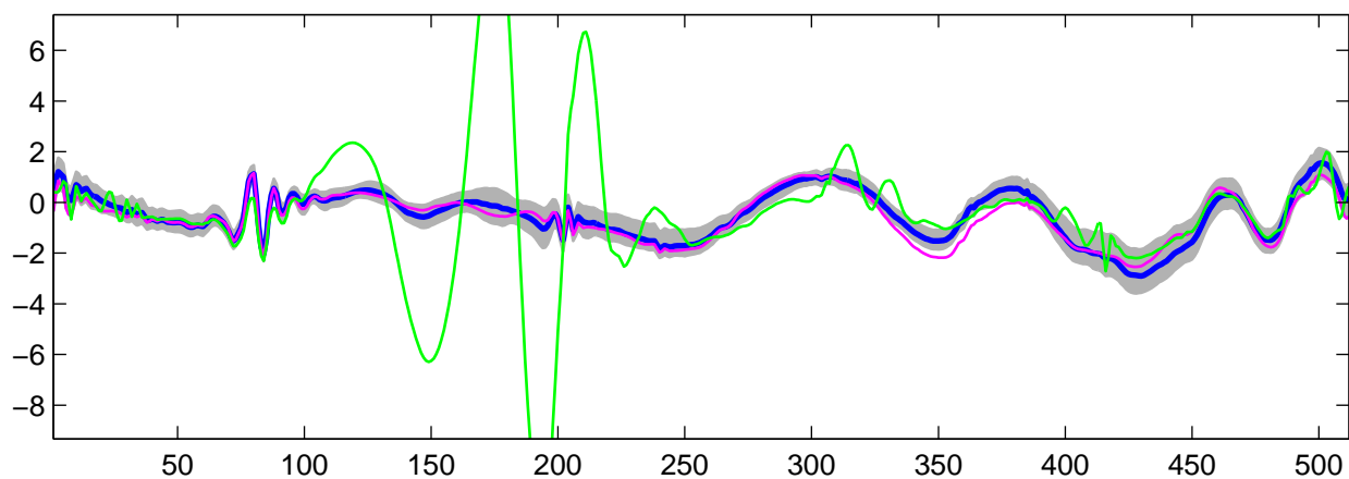
Estimated U_{24}(t) using R-WFMM: t_1 data, run 2
