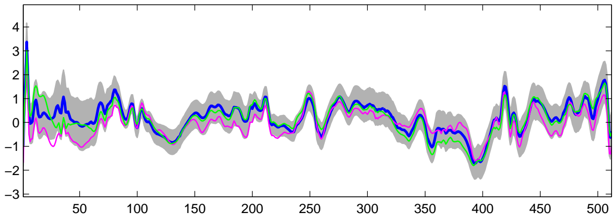
Estimated U_{25}(t) using R-WFMM: DE data, run 2
