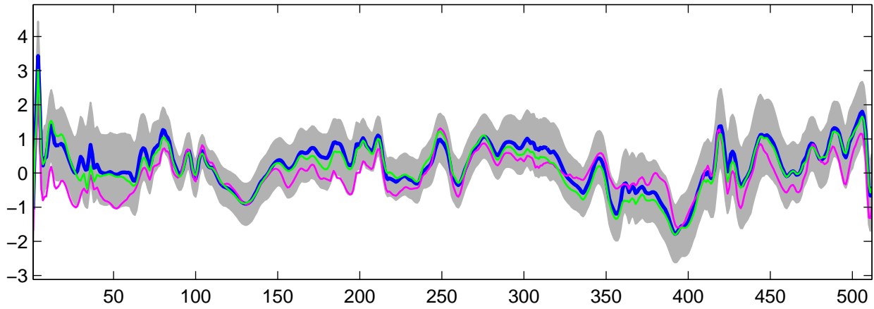
Estimated U_{25}(t) using G-WFMM: DE data, run 2
