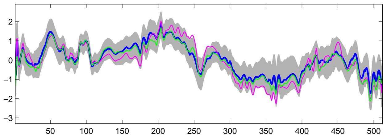
Estimated U_{25}(t) using R-WFMM: Normal data, run 2
