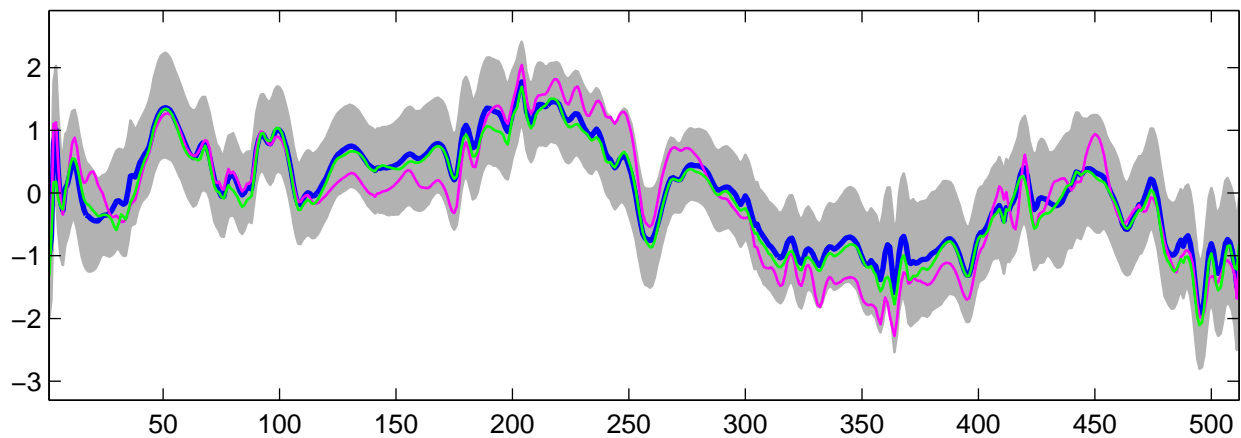
Estimated U_{25}(t) using G-WFMM: Normal data, run 2
