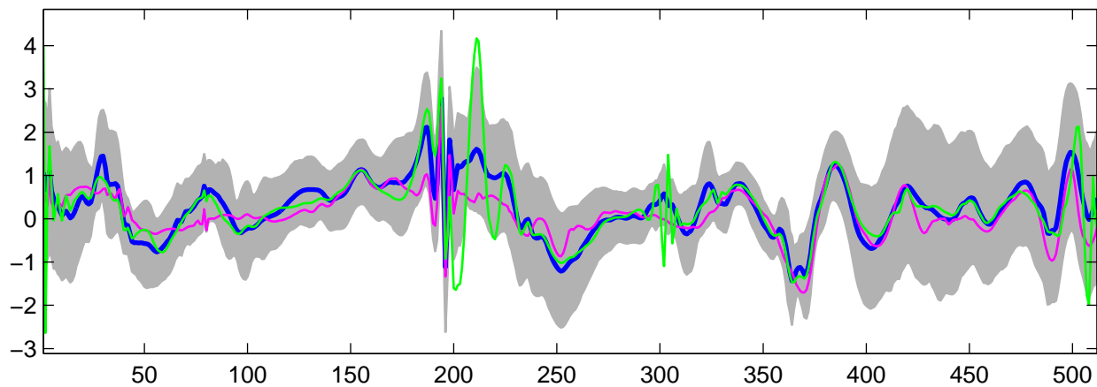
Estimated U_{25}(t) using G-WFMM: t_1 data, run 2
