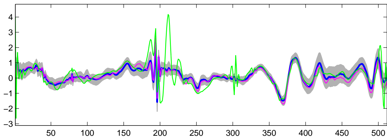
Estimated U_{25}(t) using R-WFMM: t_1 data, run 2
