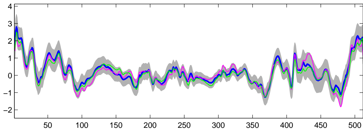
Estimated U_{25}(t) using R-WFMM: t_3 data, run 2
