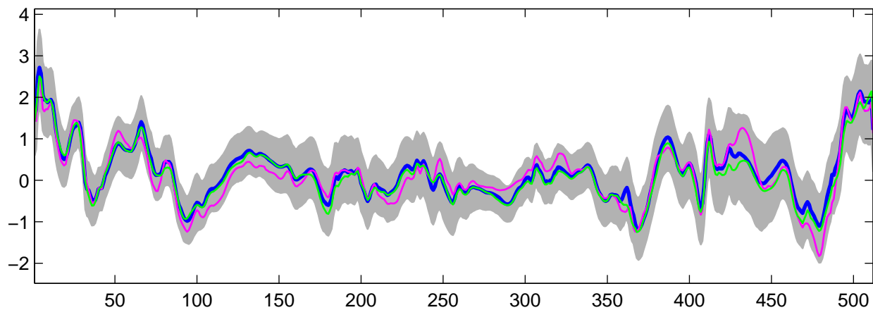
Estimated U_{25}(t) using G-WFMM: t_3 data, run 2
