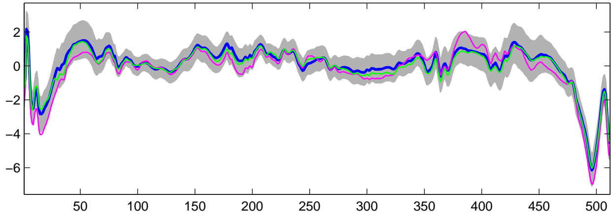
Estimated U_{26}(t) using G-WFMM: DE data, run 2
