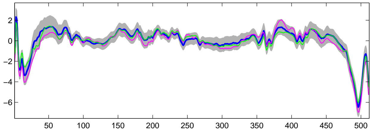
Estimated U_{26}(t) using R-WFMM: DE data, run 2
