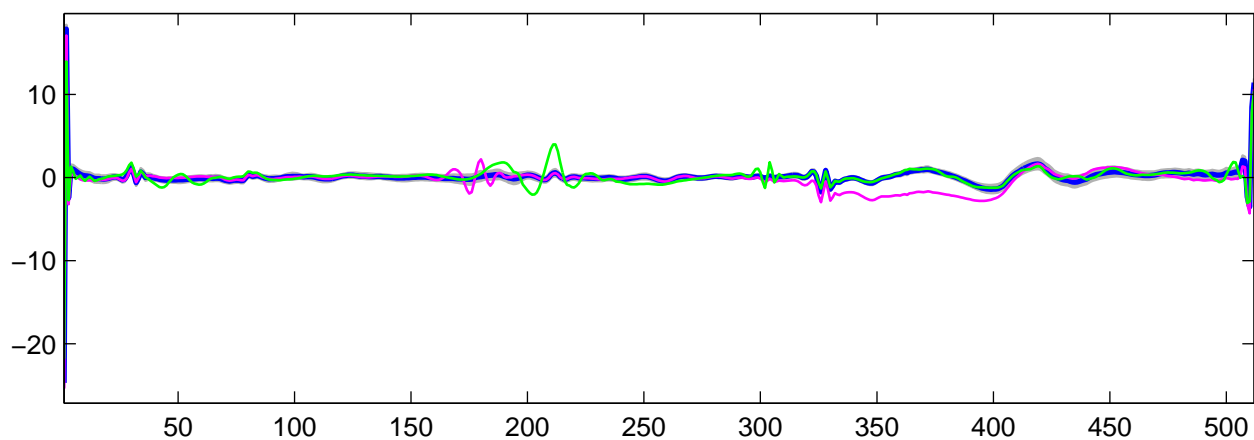
Estimated U_{26}(t) using R-WFMM: t_1 data, run 2
