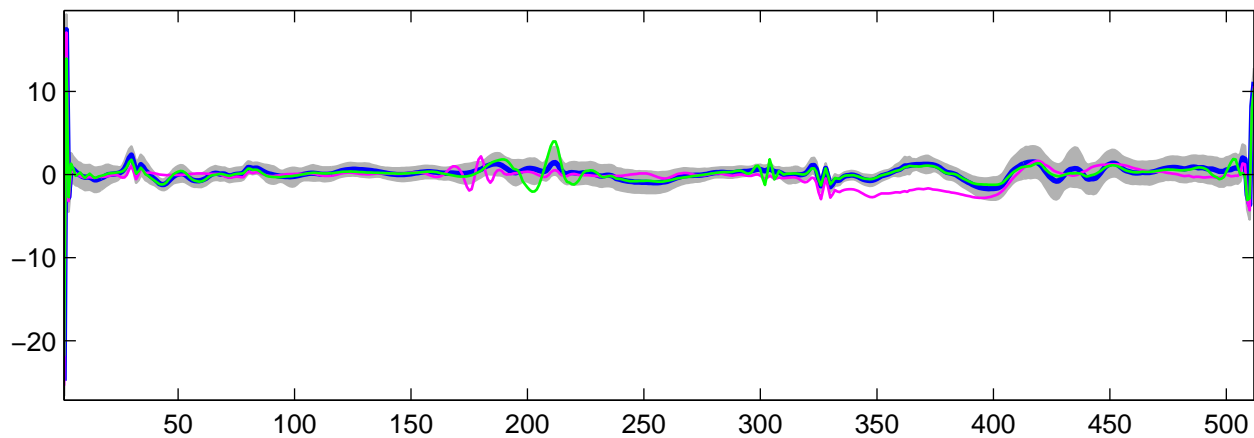
Estimated U_{26}(t) using G-WFMM: t_1 data, run 2
