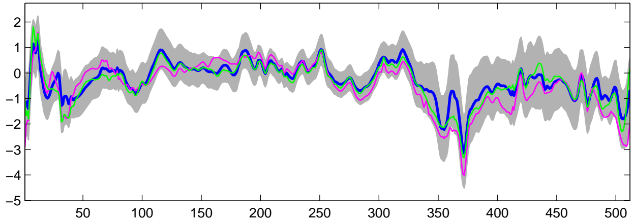
Estimated U_{26}(t) using G-WFMM: t_2 data, run 2
