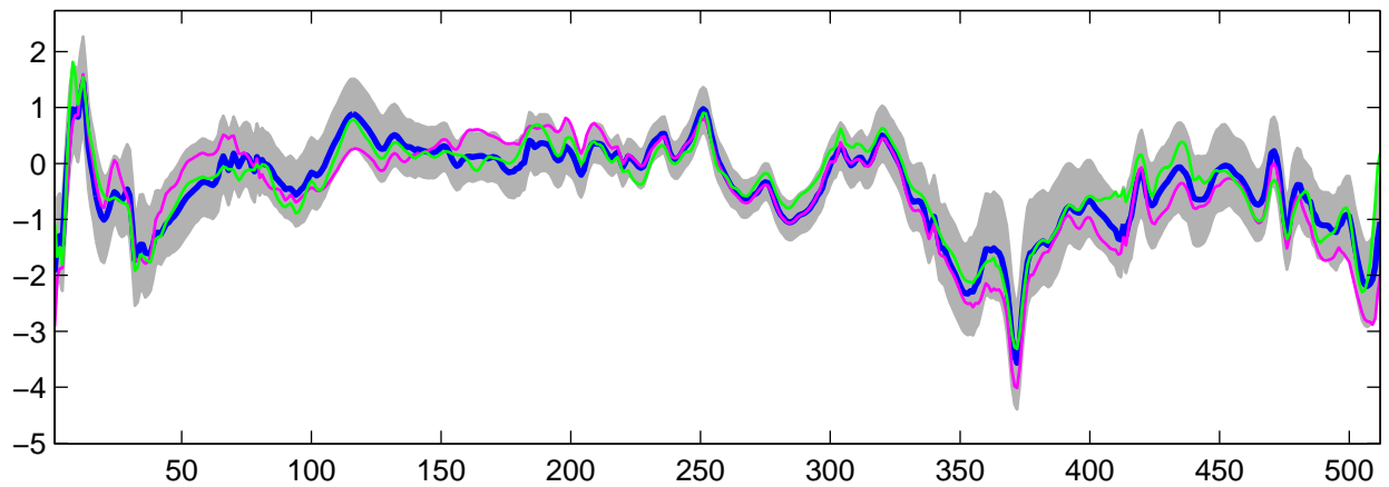
Estimated U_{26}(t) using R-WFMM: t_2 data, run 2
