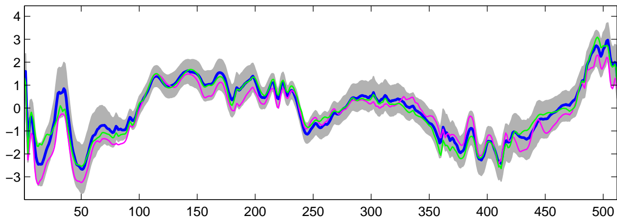
Estimated U_{27}(t) using R-WFMM: DE data, run 2
