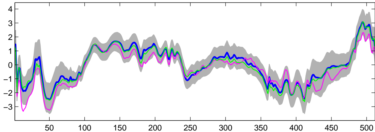
Estimated U_{27}(t) using G-WFMM: DE data, run 2
