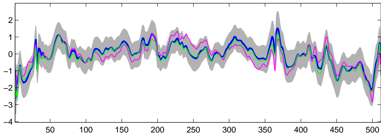
Estimated U_{27}(t) using G-WFMM: Normal data, run 2
