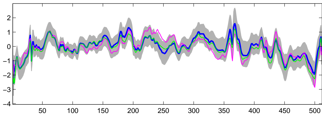
Estimated U_{27}(t) using R-WFMM: Normal data, run 2
