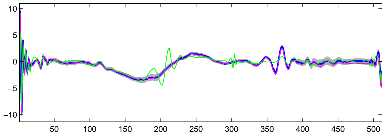
Estimated U_{27}(t) using R-WFMM: t_1 data, run 2
