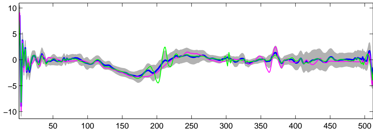
Estimated U_{27}(t) using G-WFMM: t_1 data, run 2
