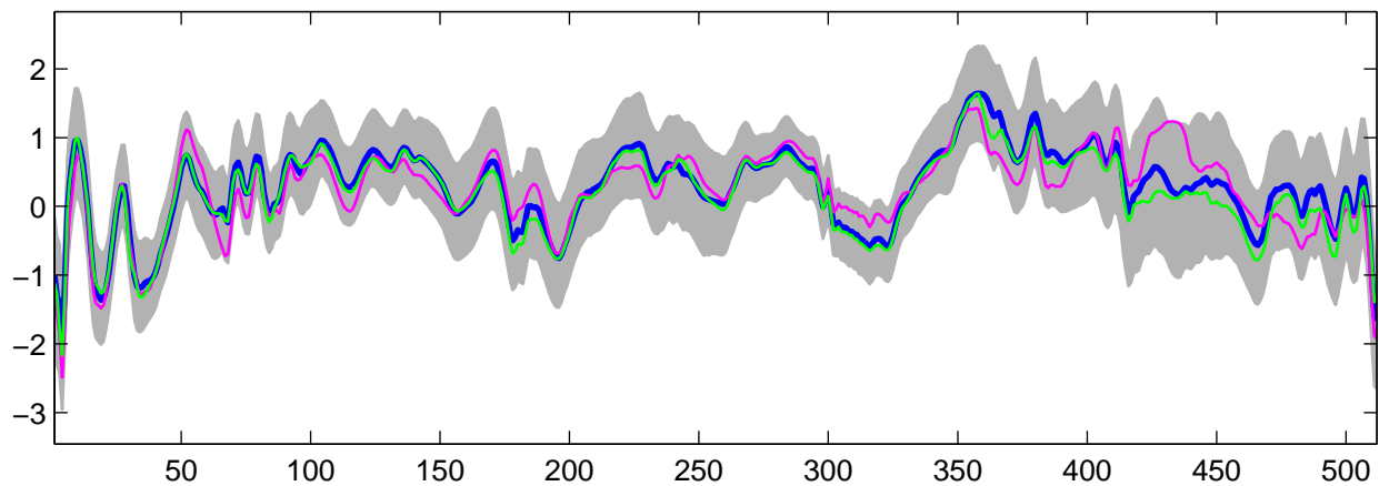
Estimated U_{27}(t) using G-WFMM: t_3 data, run 2
