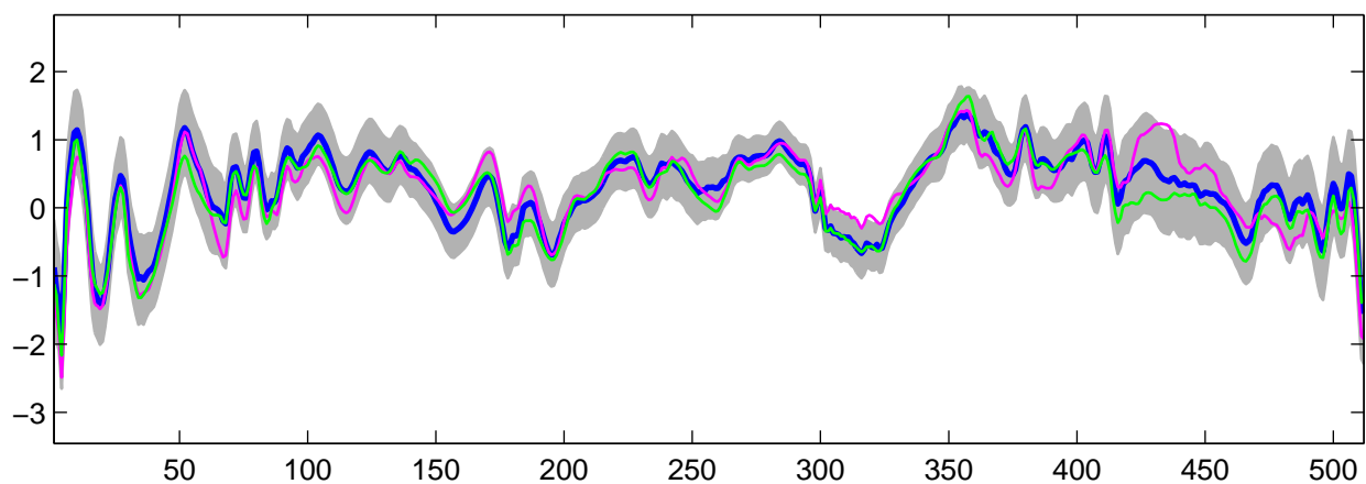
Estimated U_{27}(t) using R-WFMM: t_3 data, run 2
