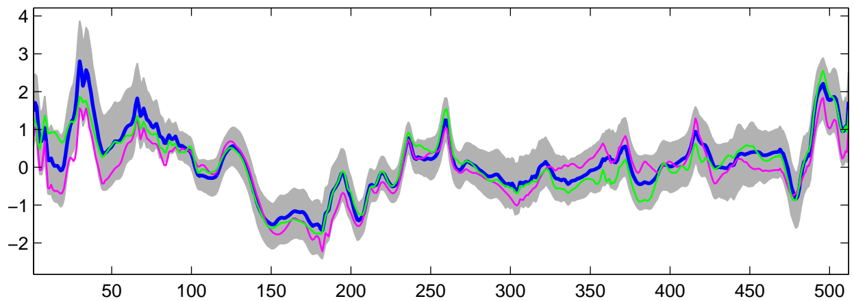
Estimated U_{28}(t) using R-WFMM: DE data, run 2
