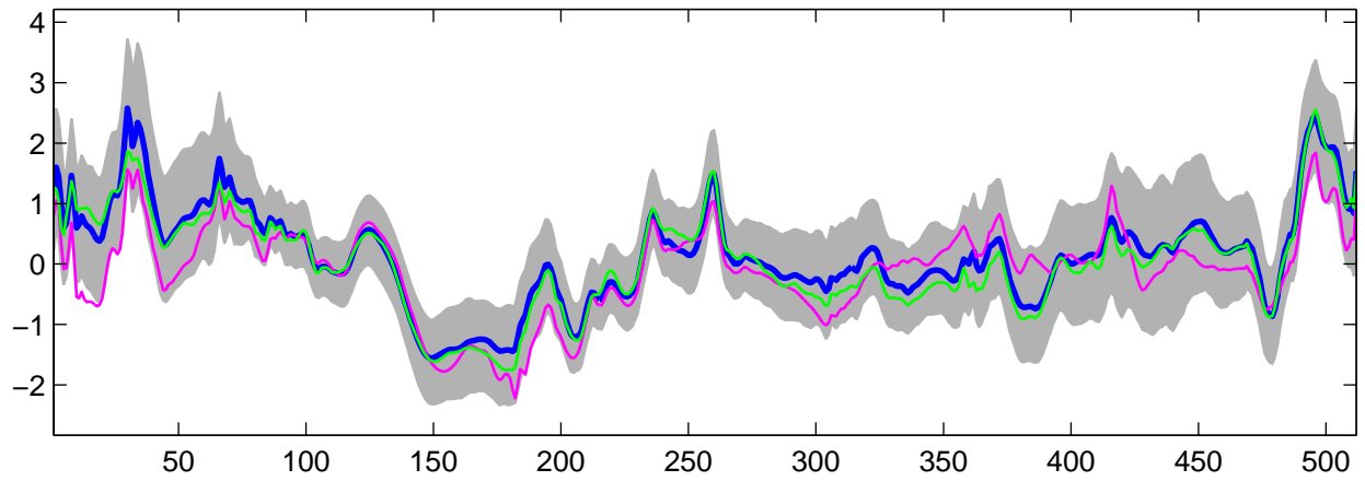
Estimated U_{28}(t) using G-WFMM: DE data, run 2
