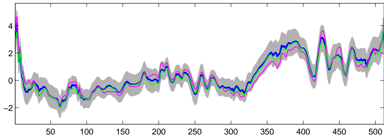
Estimated U_{28}(t) using G-WFMM: Normal data, run 2
