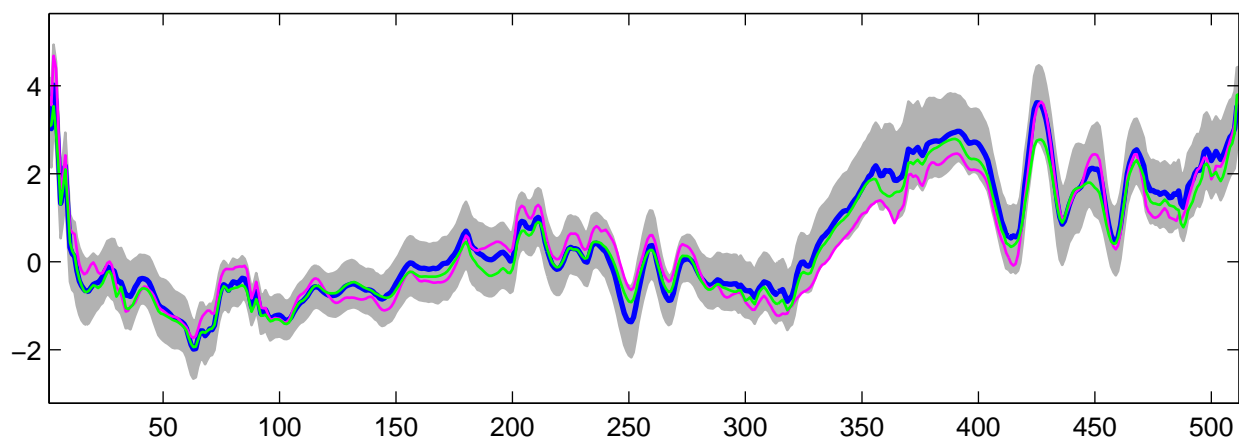
Estimated U_{28}(t) using R-WFMM: Normal data, run 2
