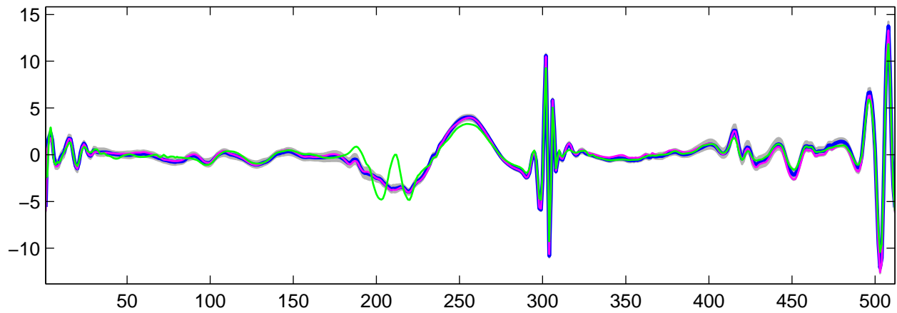
Estimated U_{28}(t) using R-WFMM: t_1 data, run 2
