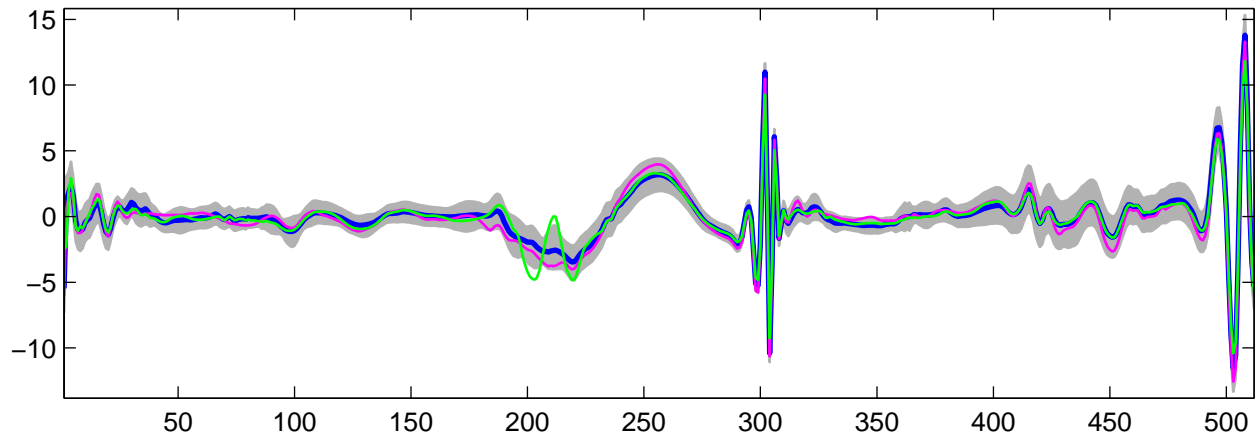
Estimated U_{28}(t) using G-WFMM: t_1 data, run 2
