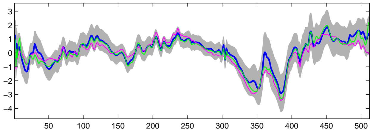
Estimated U_{28}(t) using G-WFMM: t_2 data, run 2
