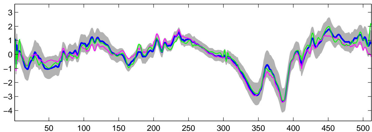
Estimated U_{28}(t) using R-WFMM: t_2 data, run 2
