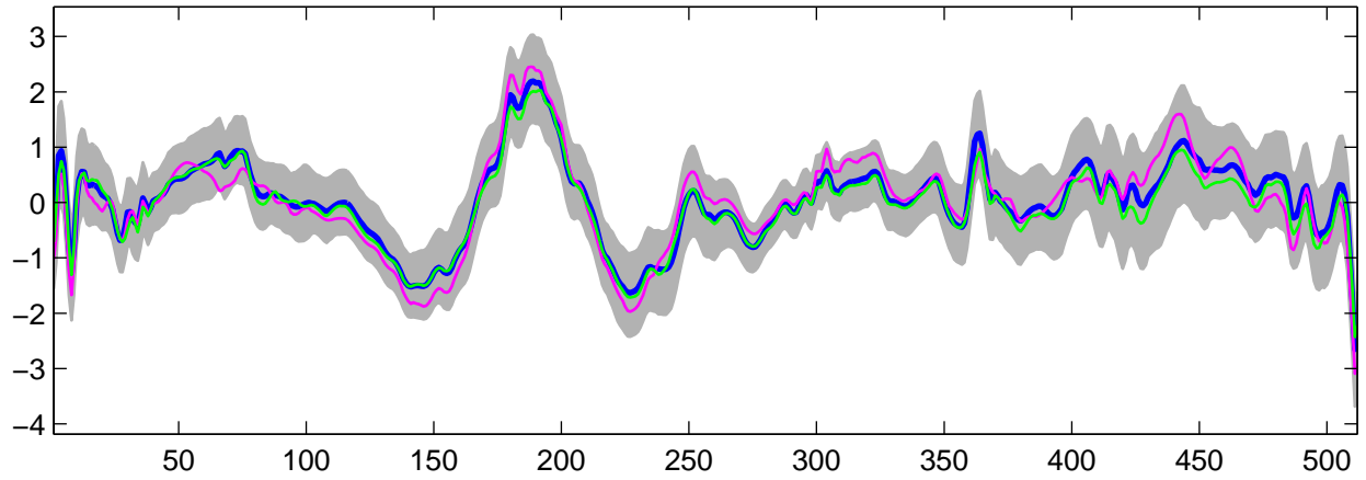
Estimated U_{28}(t) using G-WFMM: t_3 data, run 2
