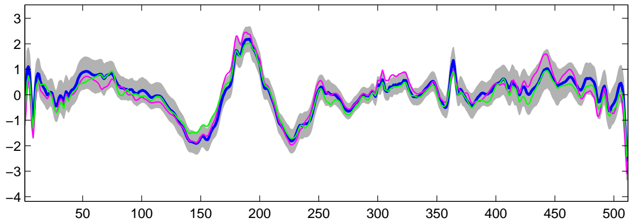
Estimated U_{28}(t) using R-WFMM: t_3 data, run 2
