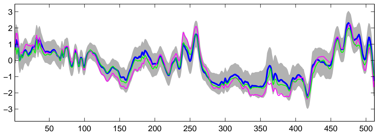
Estimated U_{29}(t) using R-WFMM: Normal data, run 2
