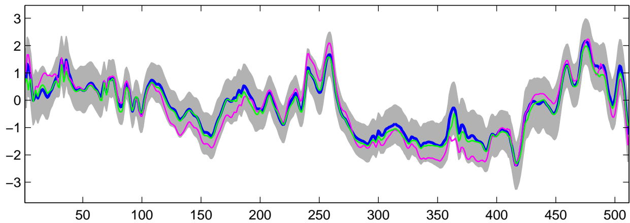
Estimated U_{29}(t) using G-WFMM: Normal data, run 2
