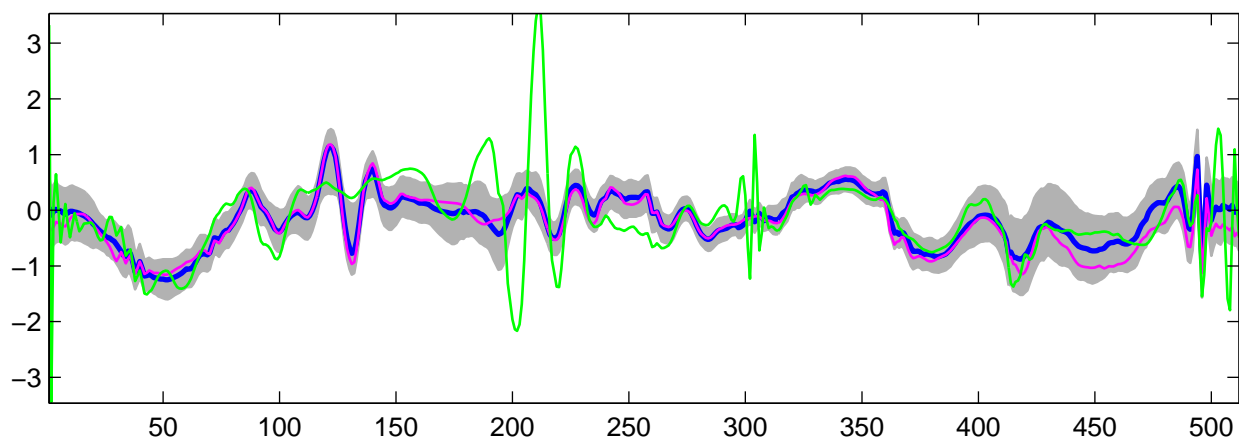
Estimated U_{29}(t) using R-WFMM: t_1 data, run 2
