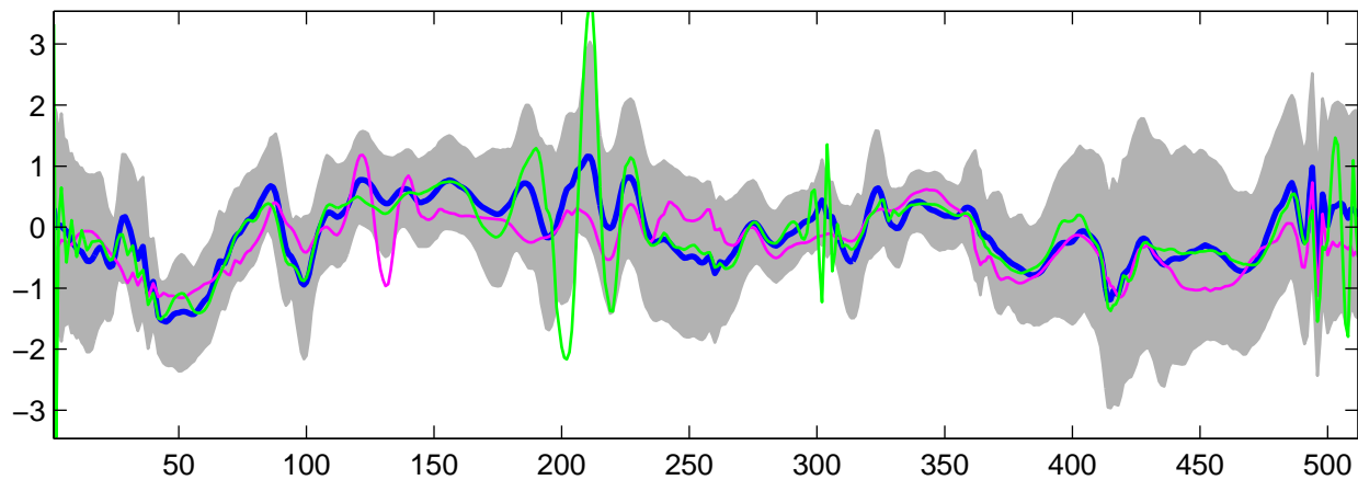
Estimated U_{29}(t) using G-WFMM: t_1 data, run 2
