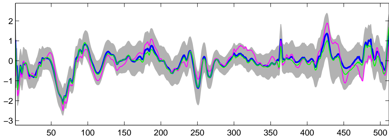
Estimated U_{29}(t) using G-WFMM: t_3 data, run 2
