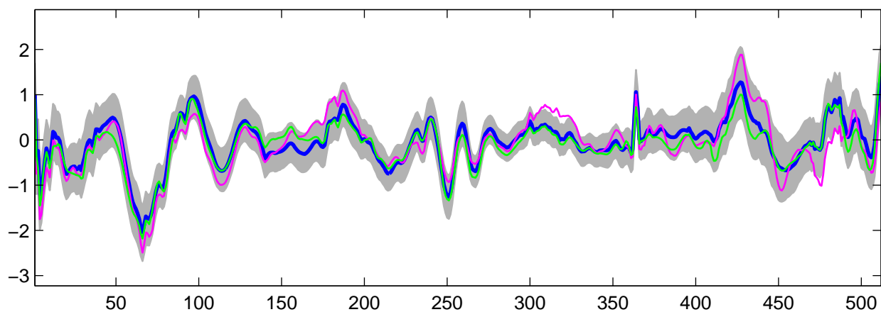
Estimated U_{29}(t) using R-WFMM: t_3 data, run 2
