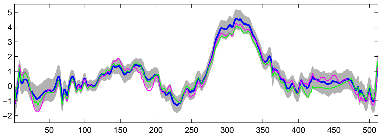
Estimated U_2(t) using R-WFMM: DE data, run 2
