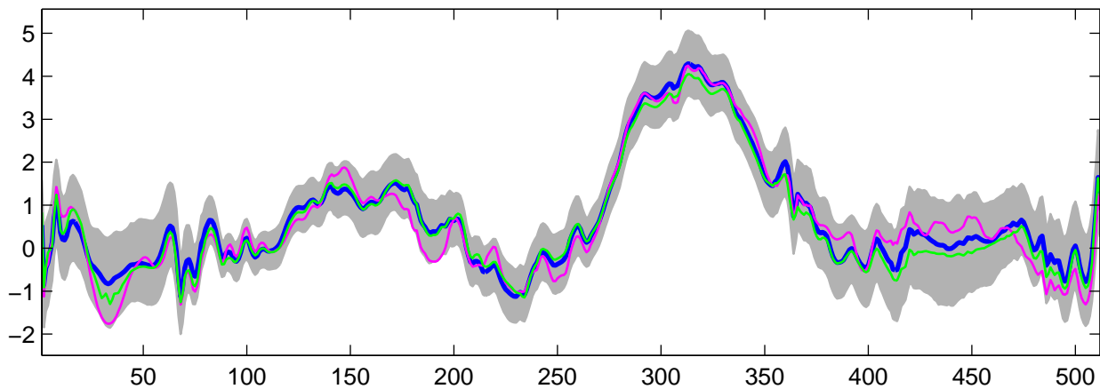
Estimated U_2(t) using G-WFMM: DE data, run 2
