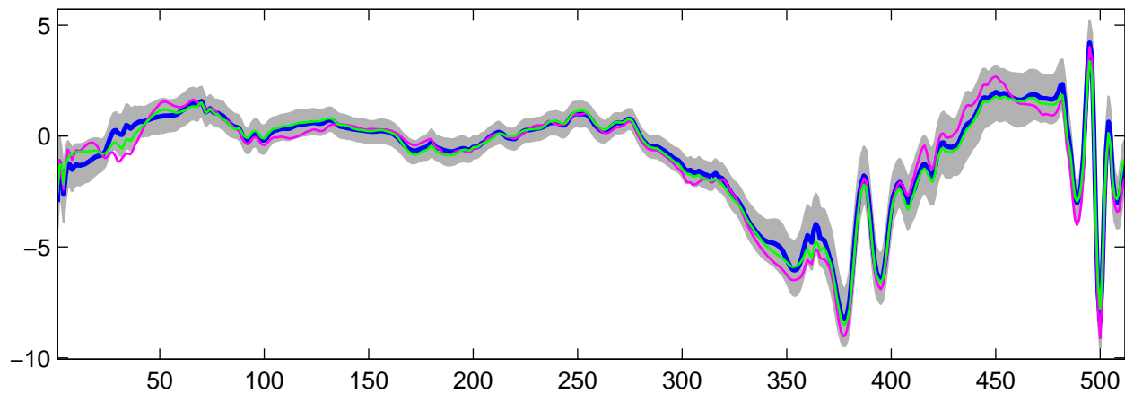
Estimated U_2(t) using G-WFMM: t_2 data, run 2
