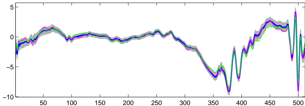
Estimated U_2(t) using R-WFMM: t_2 data, run 2
