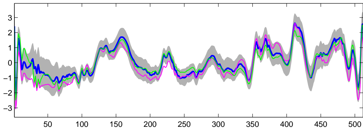
Estimated U_{30}(t) using R-WFMM: DE data, run 2
