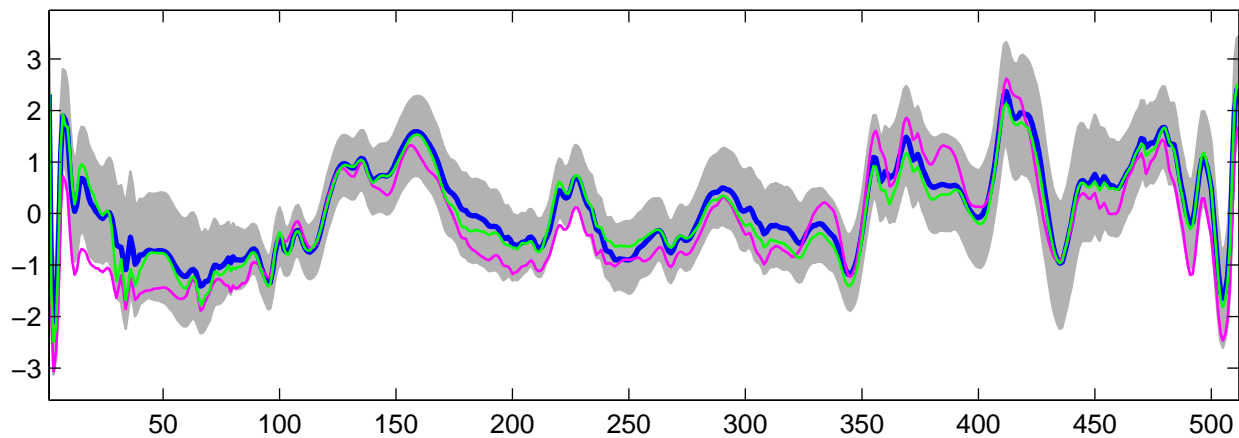
Estimated U_{30}(t) using G-WFMM: DE data, run 2
